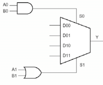
Figure 13 • C-Module Implementation
