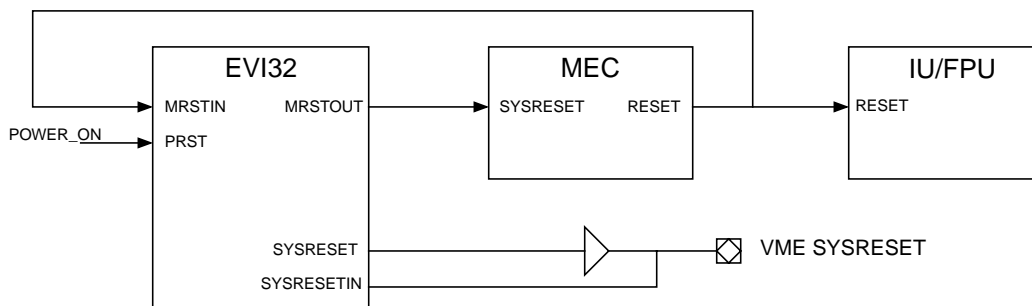
Figure 11: ERC32/EVI32 reset generation
