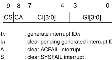
Figure 9: Interrupt command register
