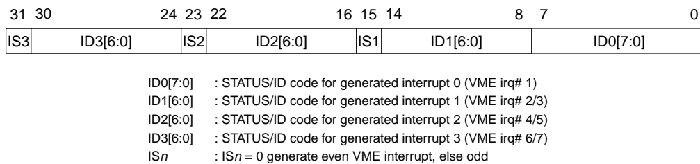
Figure 8: Interrupt identification register
